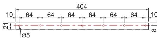
Bracket B32 (Top View)
