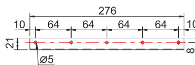
Bracket B31 (Top View)
