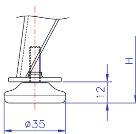
Type B With Screw Glide 10mm Height Adjustable
