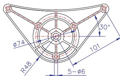
Aluminum Mounting Plate for 60mmD Steel Tube
