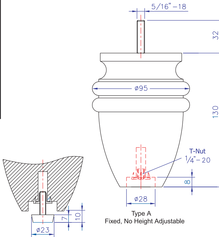
Type B Screw Glide, Thread 1/4" x 22mmL 10mm Height Adjustable
