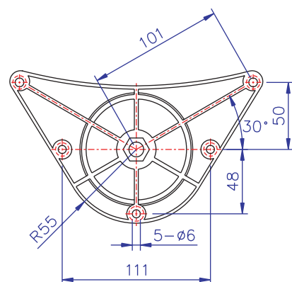
Aluminum Mounting Plate for 80mmD Steel Tube
