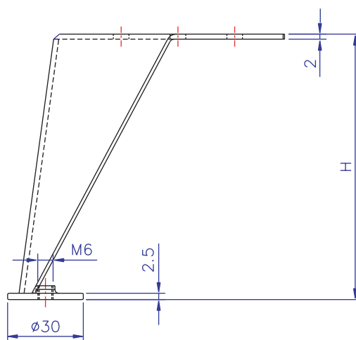
Type A Without Screw Glide
