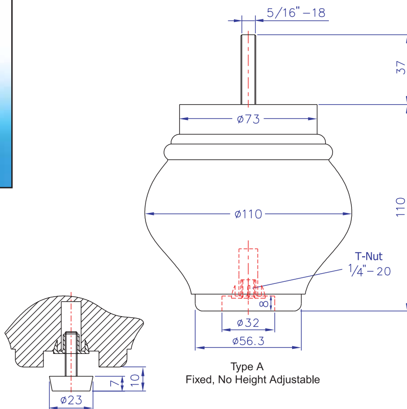
Type B Screw Glide, Thread 1/4" x 22mmL 10mm Height Adjustable
