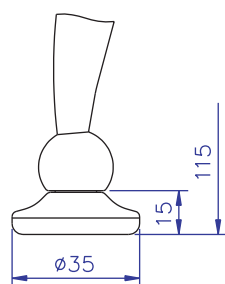
Type B With Screw Glide 10mm Height Adjustable
