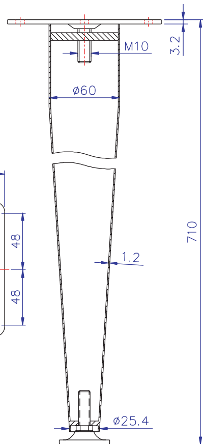
Screw Glide #9210-30 15mm Height Adjustment
