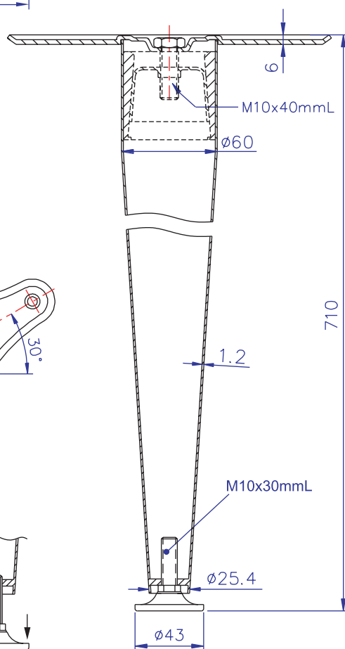
Screw Glide #9210-30 15mm Height Adjustment
