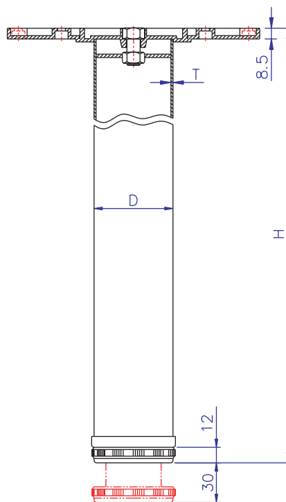
Aluminum Mounting Plate for 80mmD Steel Tube
