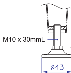
Screw Glide #9210-30 15mm Height Adjustment
